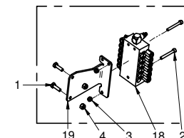
DIVIDER FIXING
