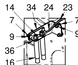
DETAIL J
