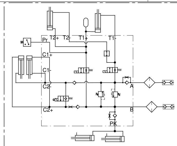
HYDRAULIC DIAGRAM
