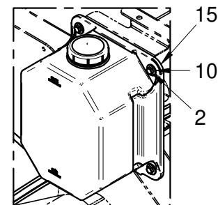
DETAIL H
